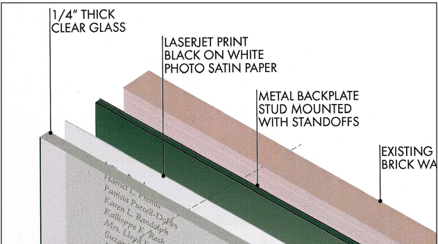
Sandwich detail
